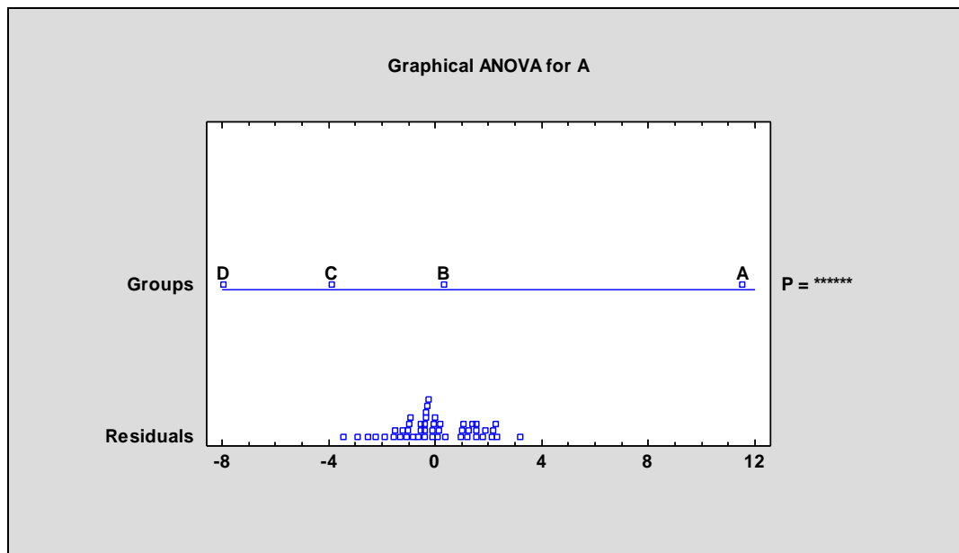
Figure 13-8. Graphical ANOVA
