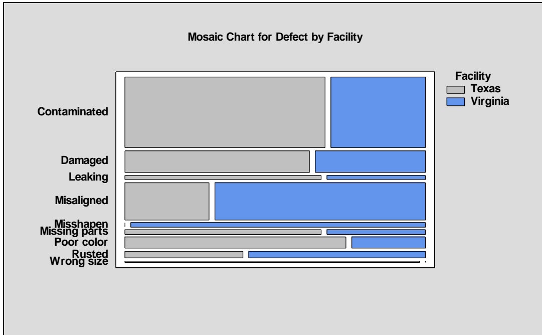
Figure 15-12. Mosaic Plot
