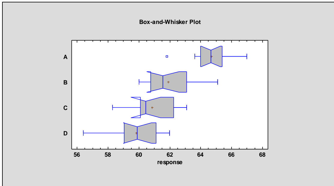
Figure 13-12. Box-and-Whisker Plots with Median Notches
