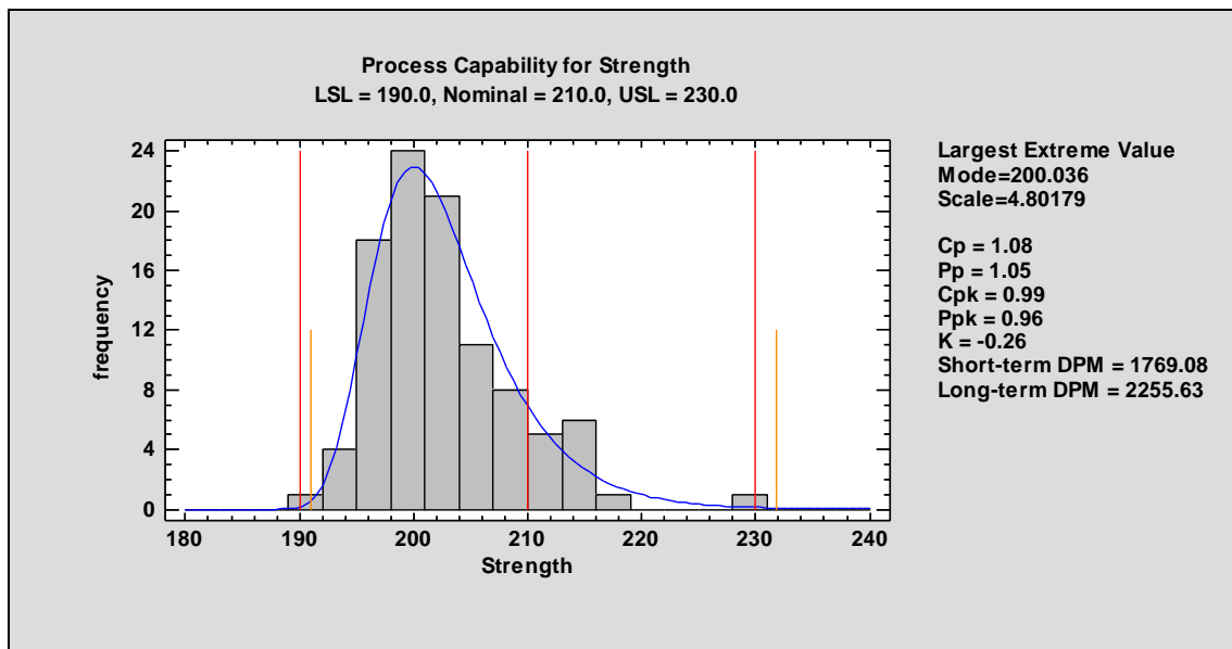
Figure 16-10. Fitted Largest Extreme Value Distribution
