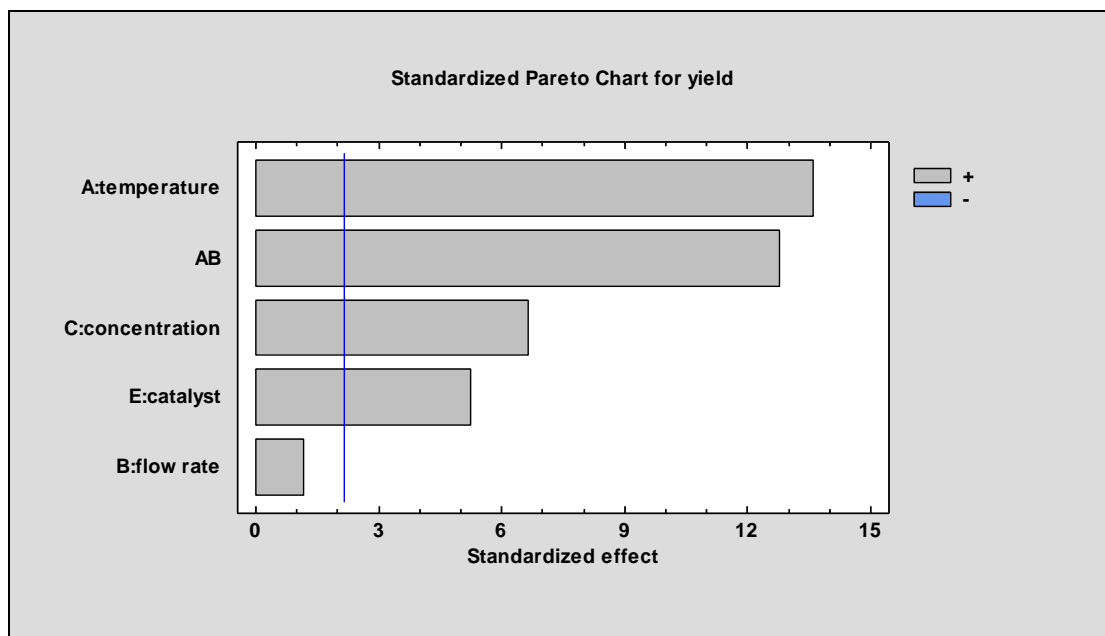
Figure 17-22. Standardized Pareto Chart after Removing Effects
