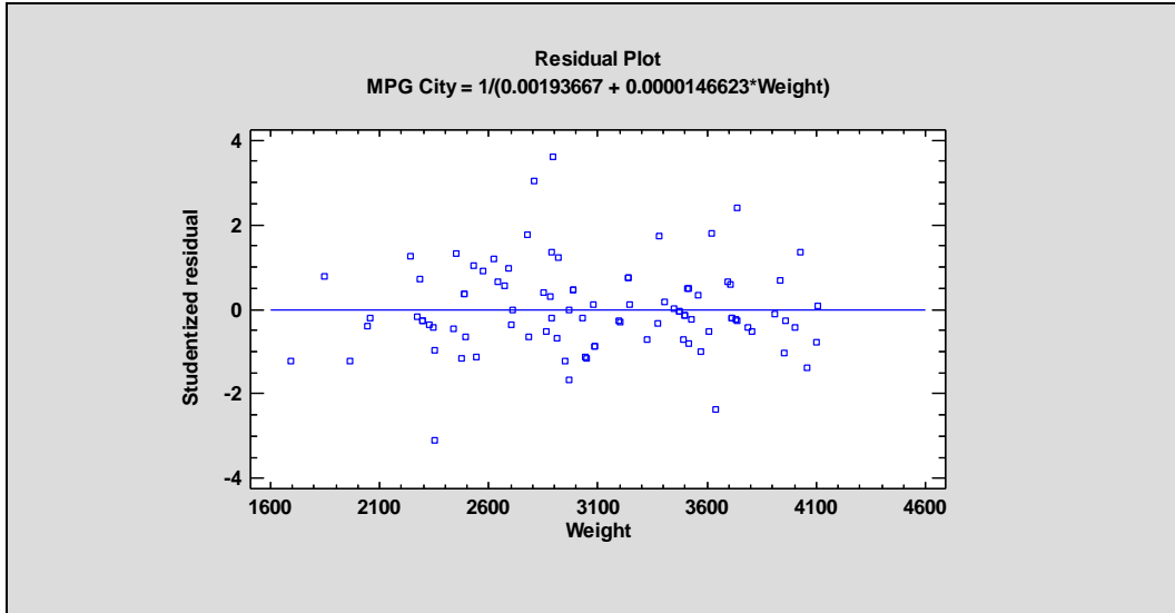
Figure 14-13. Plot of Studentized Residuals
