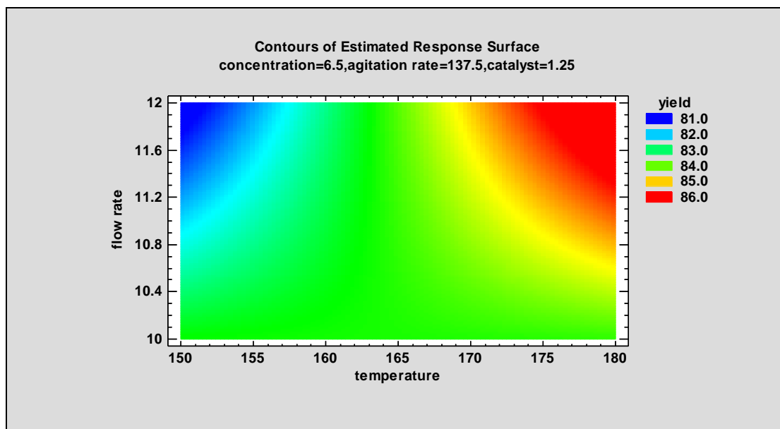
Figure 17-28. Contour Plot of Response Surface for Yield
