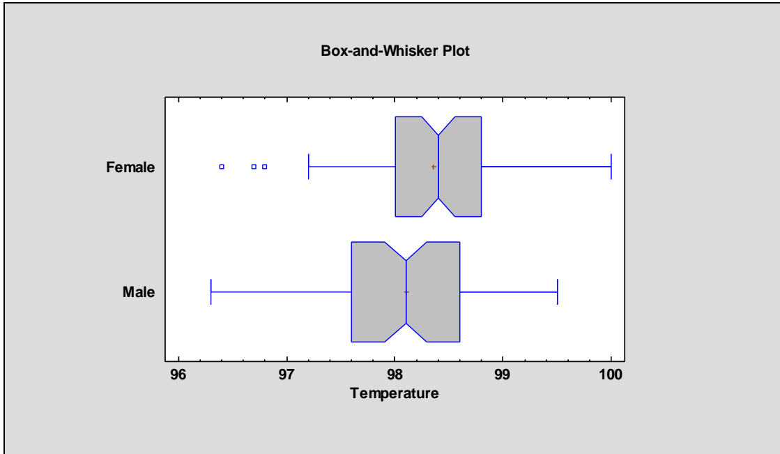
Figure 12-5. Dual Box-and-Whisker Plot with Median Notches
