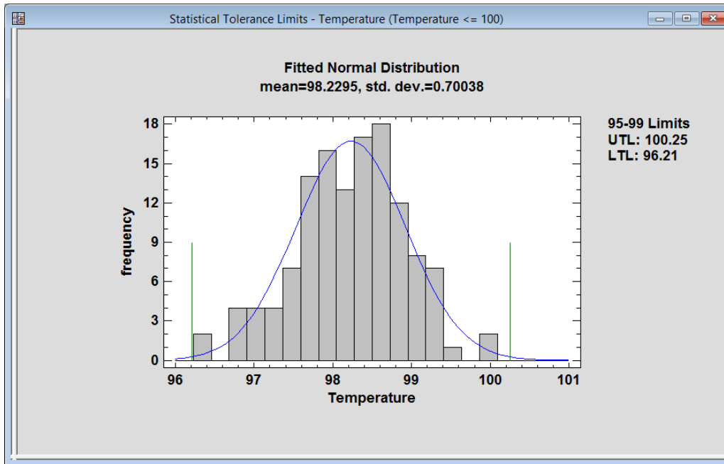
Figure 11-29. Tolerance Plot
