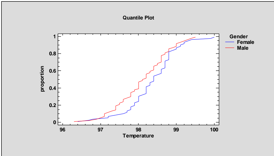
Figure 12-9. Side-by-Side Quantile Plots
