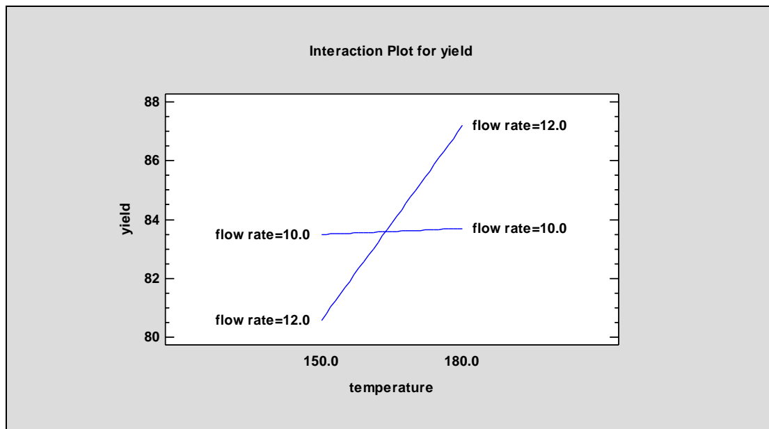
Figure 17-20. Interaction Plot for Flow Rate and Temperature
