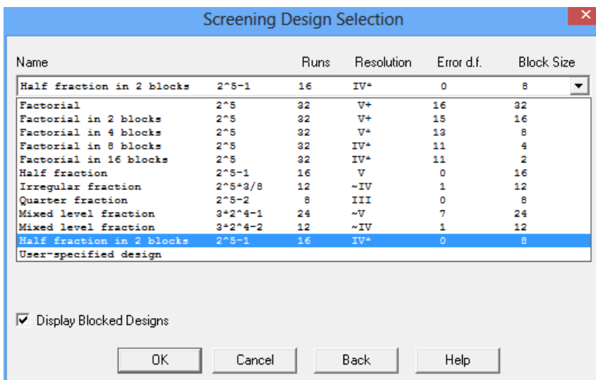
Figure 17-6. Design Selection
