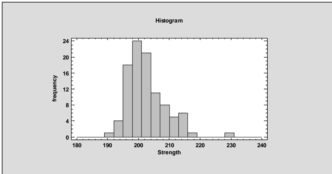
Figure 16-2. Frequency Histogram
