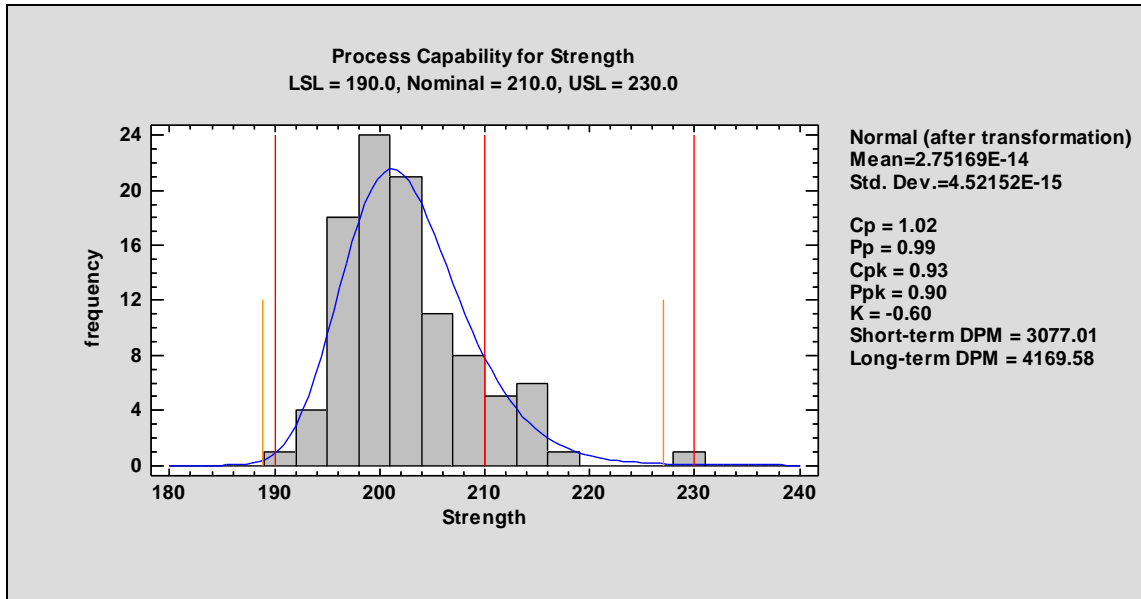
Figure 16-13. Capability Plot after Box-Cox Transformation
