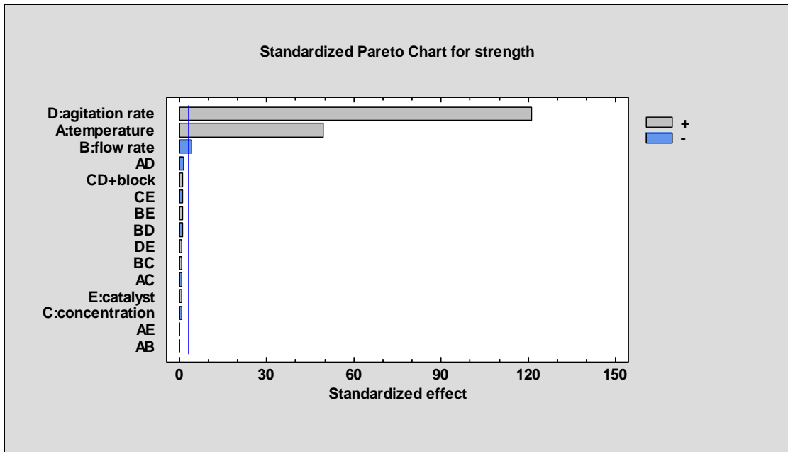
Figure 17-29. Standardized Pareto Chart for Strength
