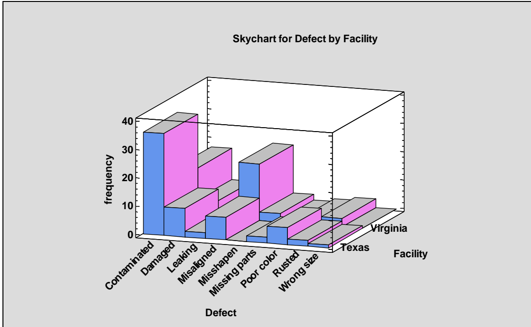
Figure 15-13. Three-Dimensional Skychart
