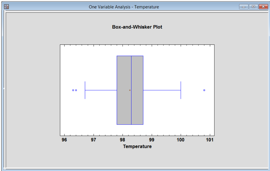
Figure 11-8. Box-and-Whisker Plot for Body Temperatures
