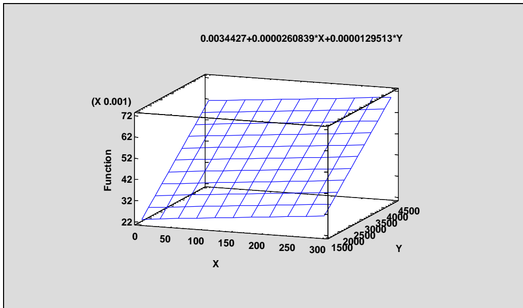
Figure 14-20. Surface Plot with Default Labels and Scaling
