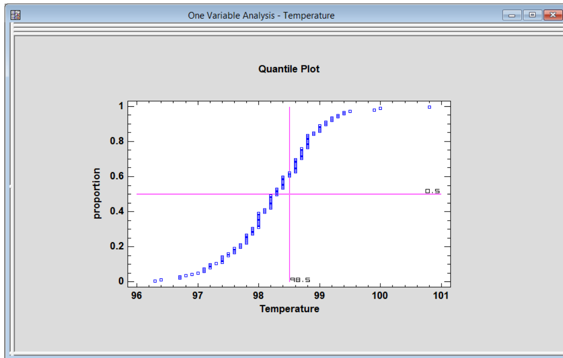
Figure 11-19. Quantile Plot
