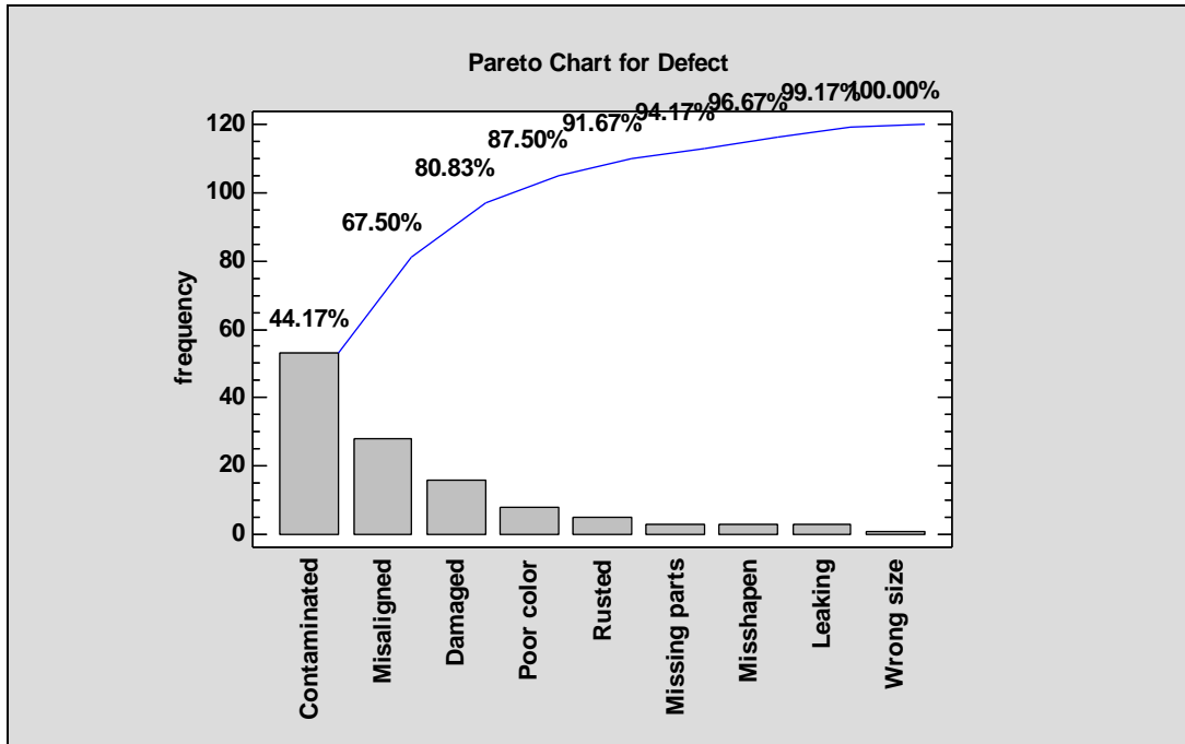
Figure 15-5. Enlarged Pareto Chart
