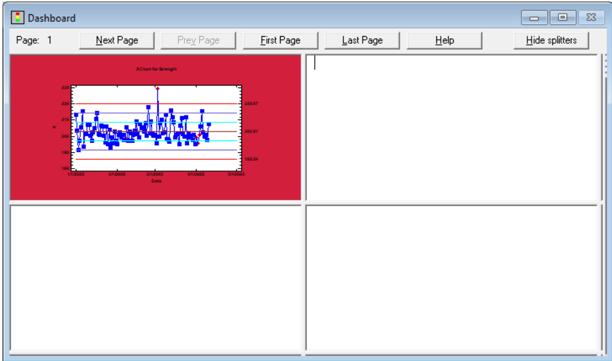
Figure 8-4. X Chart in Dashboard Window
