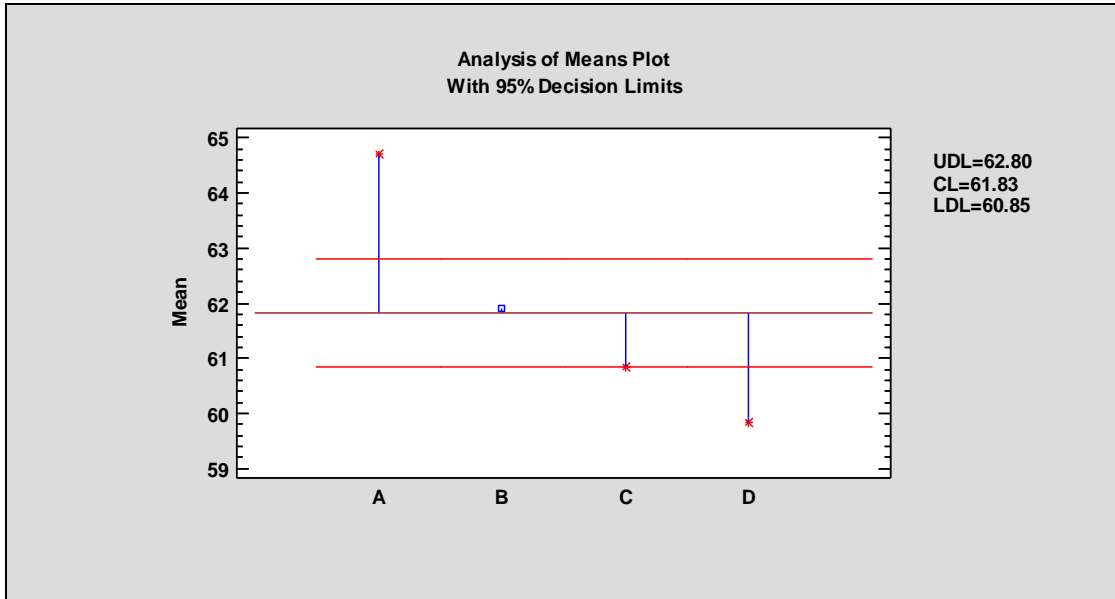
Figure 13-15. Analysis of Means Plot
