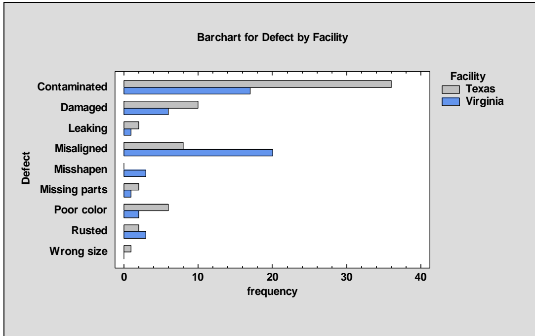
Figure 15-11. Clustered Barchart
