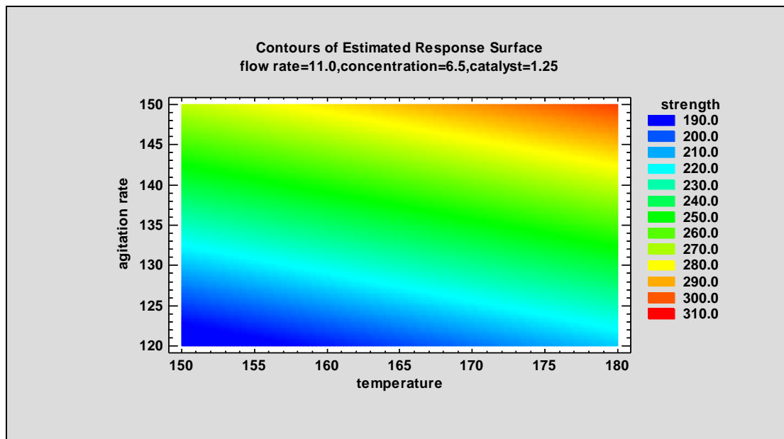
Figure 17-30. Contour Plot of Response Surface for Strength
