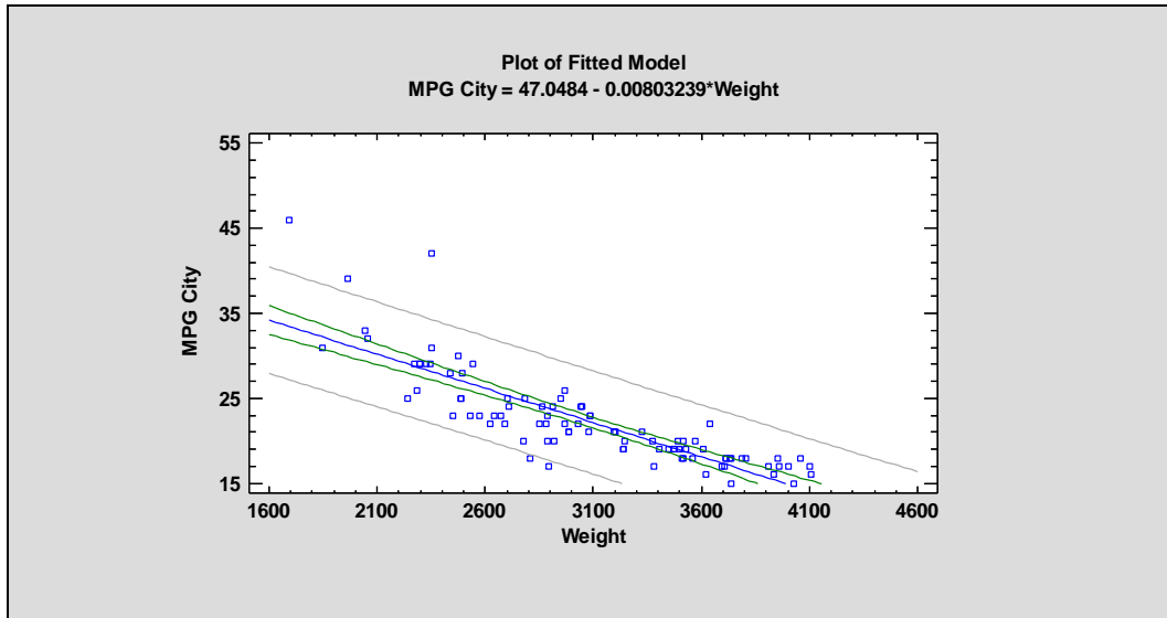
Figure 14-10. Plot of Fitted Linear Model
