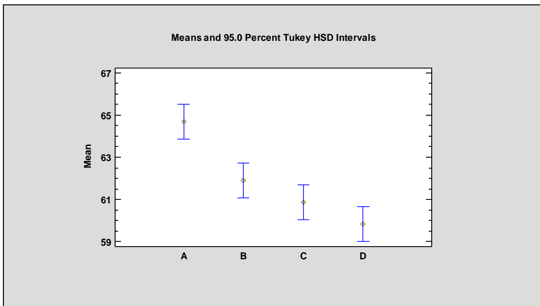
Figure 13-9. Means Plot
