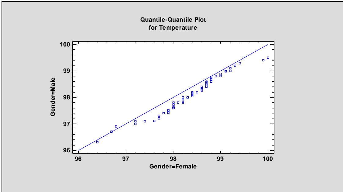
Figure 12-11. Q-Q Plot of Body Temperature Data
