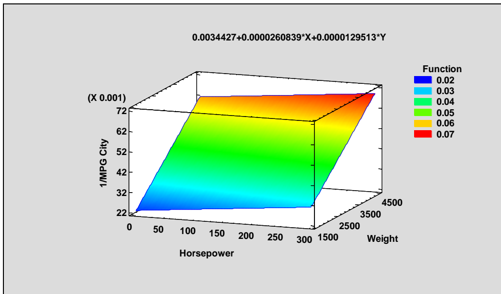
Figure 14-22. Plot of Fitted Model
