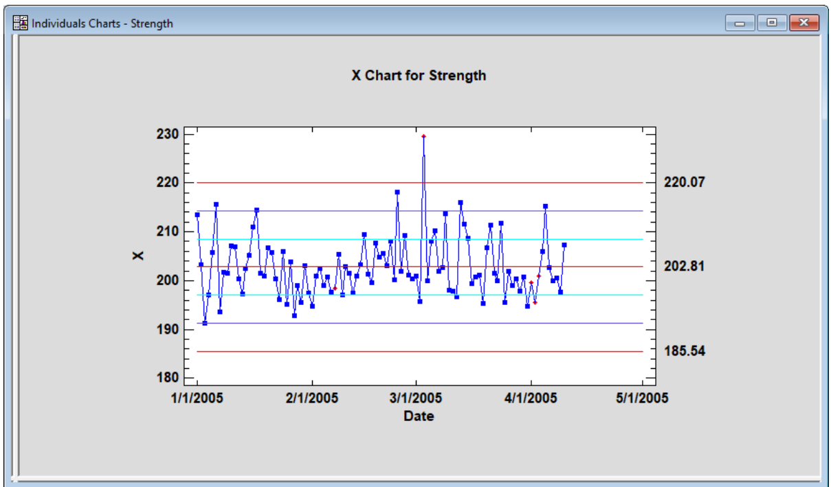
Figure 8-3. X Chart for SPC Data
