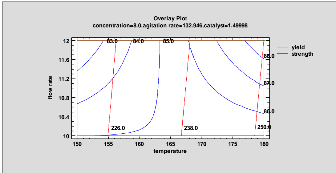
Figure 17-35. Overlaid Contour Plots for the Two Responses
