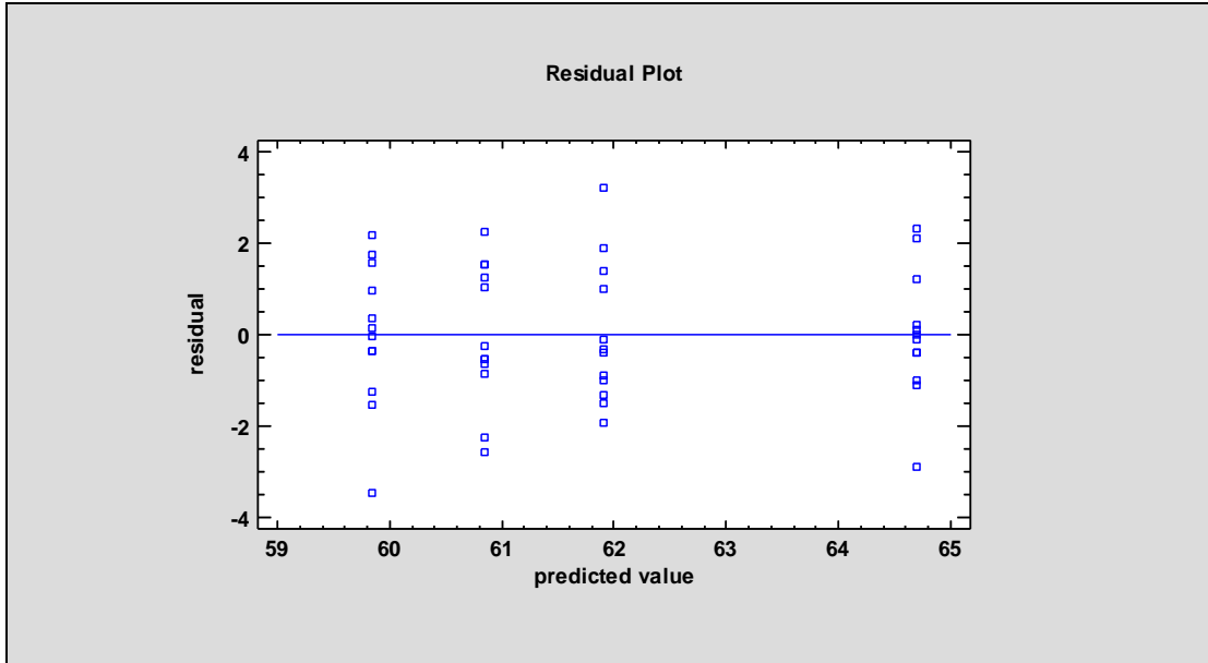
Figure 13-14. Plot of residuals Versus Predicted Strength
