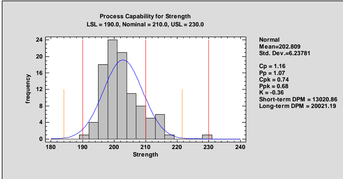
Figure 16-5. Capability Plot with Normal Distribution
